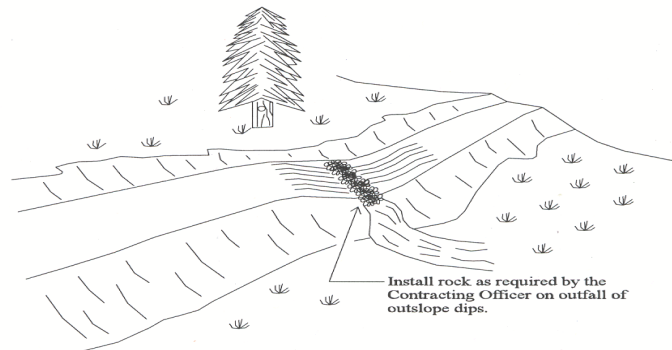
Typical Water Dip
