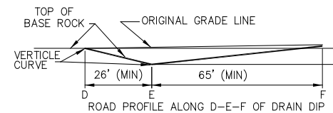
ROAD PROFILE ALONG D-E-F OF DRAIN DIP
