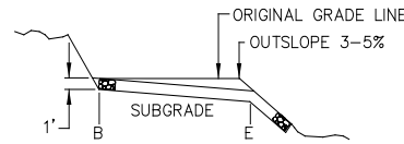
ROCK SPILL APRON 15' WIDE WITH MATERIAL AS SHOWN ON SCHEDULE OF ITEMS TO TOE OF FILL.
