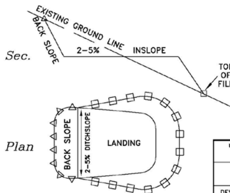
TYPICAL LANDING CUT AND FILL
