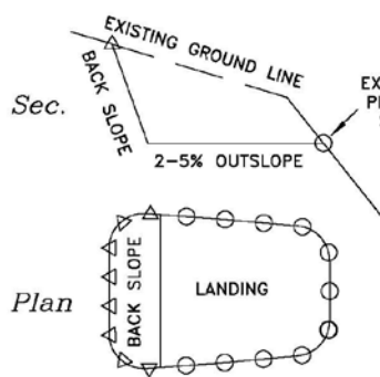
TYPICAL LANDING CUT ONLY
